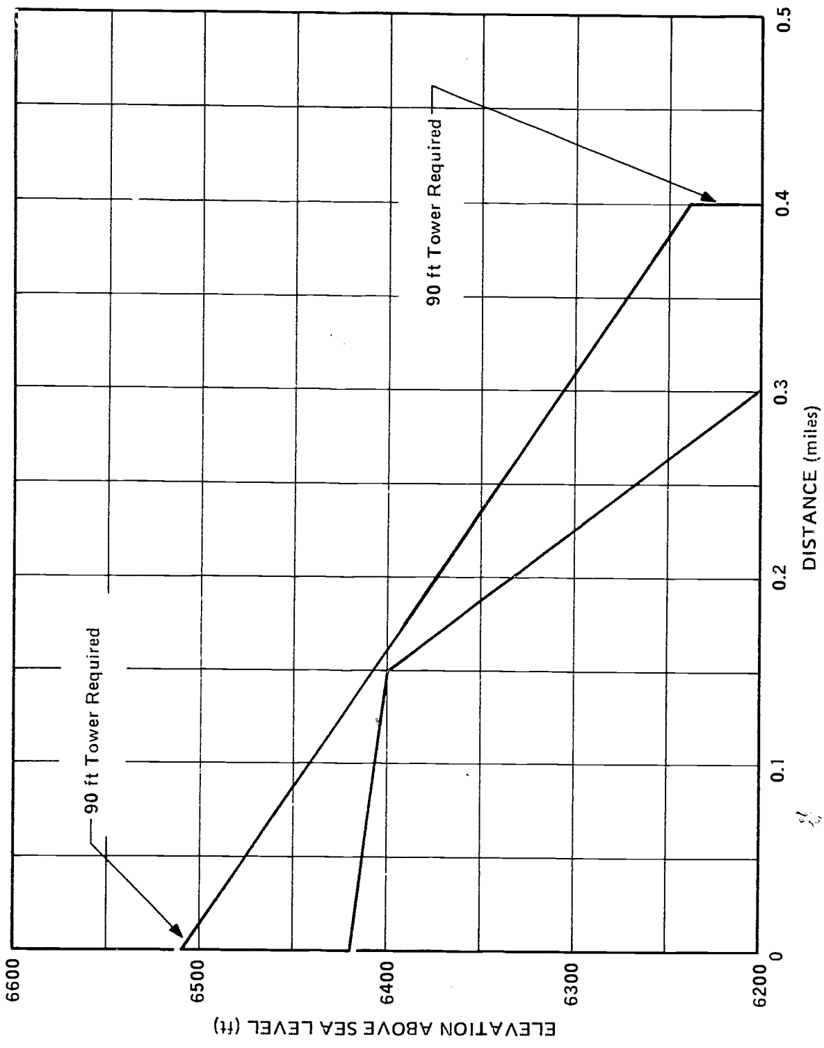
Figure A.65. Microwave Path Profile, Keams Canyon Repeater to Keams Canyon.
