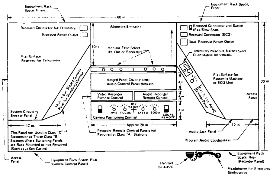
Figure 8.5. Typical Control Console.
