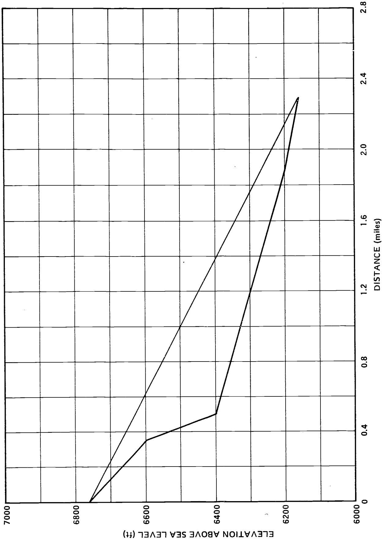
Figure A.68. Microwave Path Profile, Low Mountain Repeater to Low Mountain.
